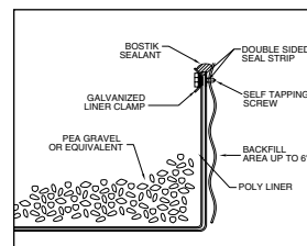
Polyliner Detail
